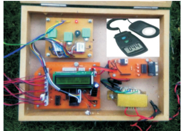
Figure 13. Experimental Setup for Calibration of System for Light Intensity
