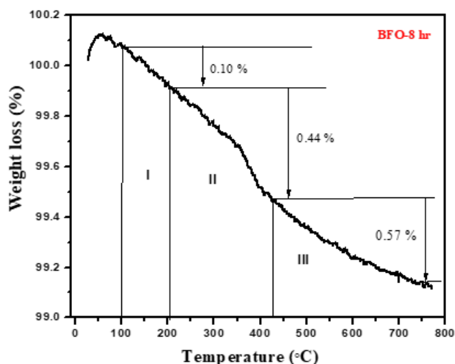
Fig 3.4 TGA curve of BFO sample annealed at 600 °C for 8 hr
