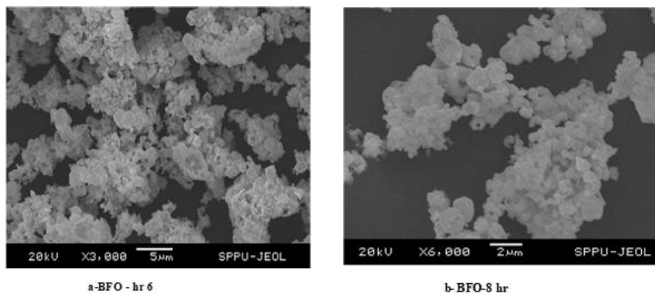
Fig 3.3 SEM images and EDS spectrum of BFO sample annealed at 600\text{ }^{\circ}\text{C} a) 6 hr b) 8 hr
