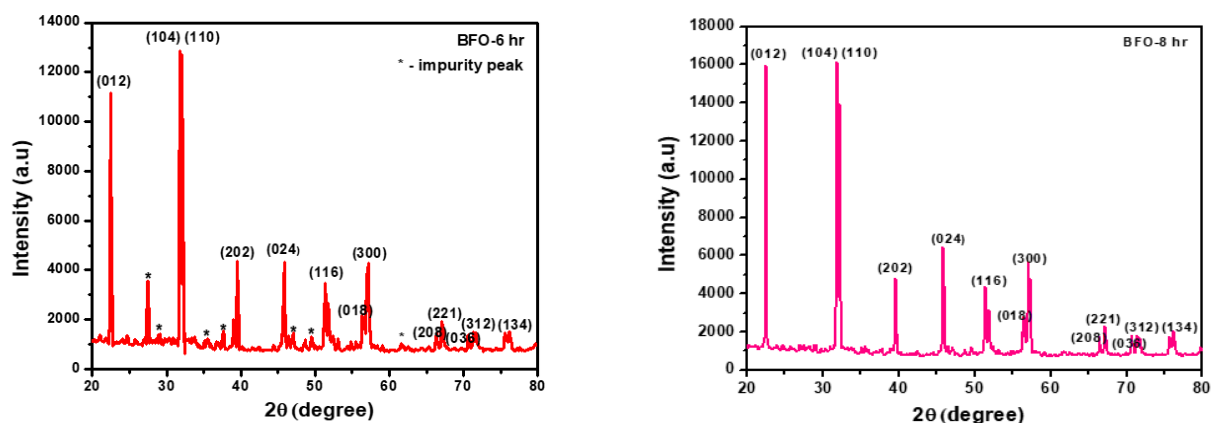
Fig 3.1 XRD pattern of BFO sample annealed at 600\text{ }^{\circ}\text{C} for 6 hr and 8 hr
