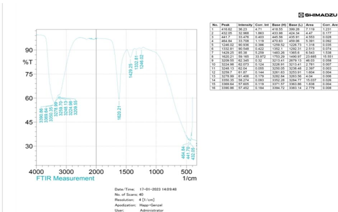
Figure: 9 - FTIR (dissolution of SF in \text{ZnCl}_2 56% w/v)
