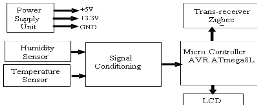
Figure 1: Block diagram of Wireless Sensor Node (WSNode)
