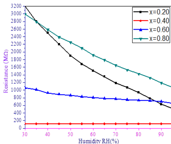
Figure 4: Graph of Resistance ( R_H ) against applied relative humidity (RH%)
