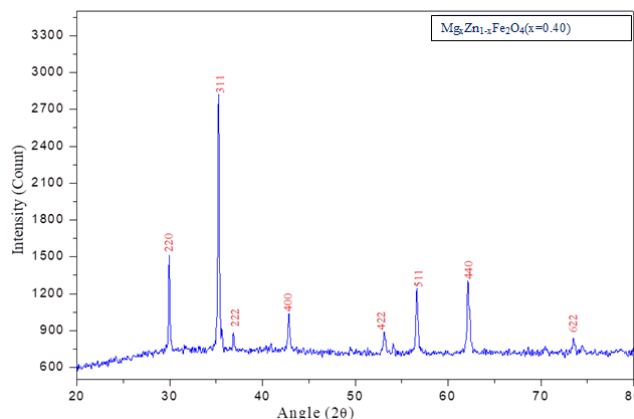
Figure 1: Typical X- ray Diffractogram for the composition ( x=0.40 )
