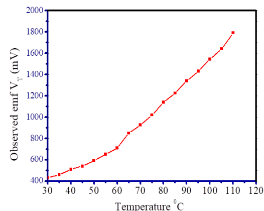
Figure 8: The Graph of Observed emf ( V_T ) in mV against applied Temperature in °C
