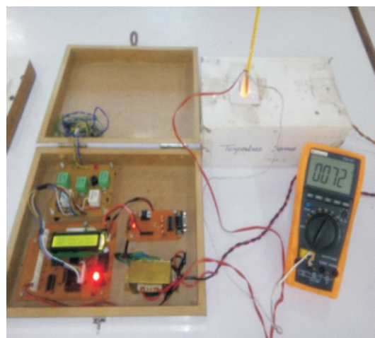
Figure 9. Calibration of System for Temperature
